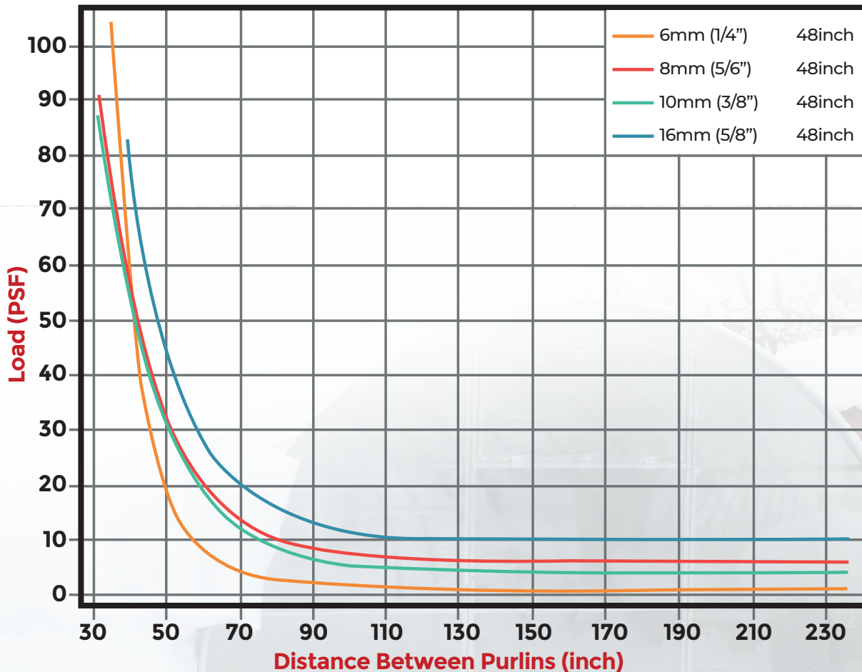
Load vs. Distance Between Purlins at an Absolute Deflection of 2 inch and various Rafters Distance
